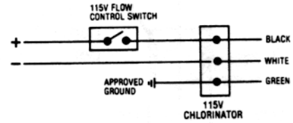
Figure 8 Wiring Diagram 115 V Chlorinator Flow Switch Operated
